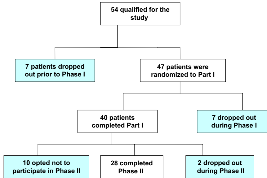
Fig. 2. Study algorithm.
